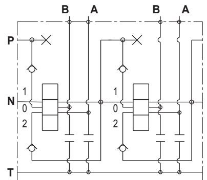
Series circuit pre-arranged for aux. valve
