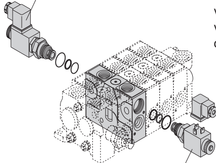
Electric venting valve
