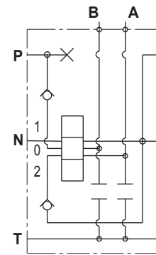
Series circuit pre-arranged for aux. valve
